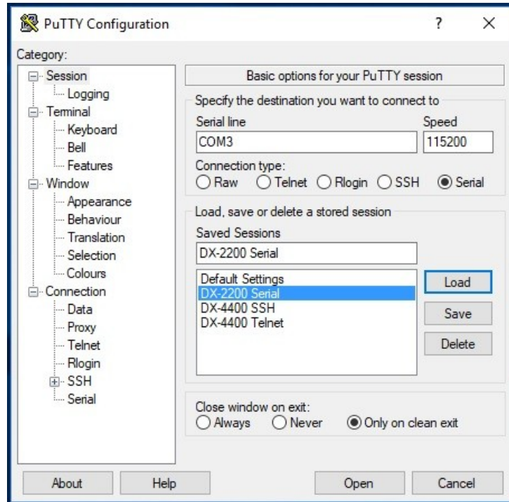
Figure 71: PuTTY Serial Port Session Settings
