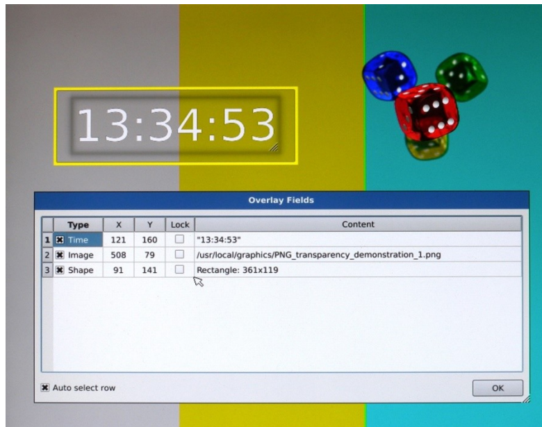
Figure 66: Overlay Fields Window
