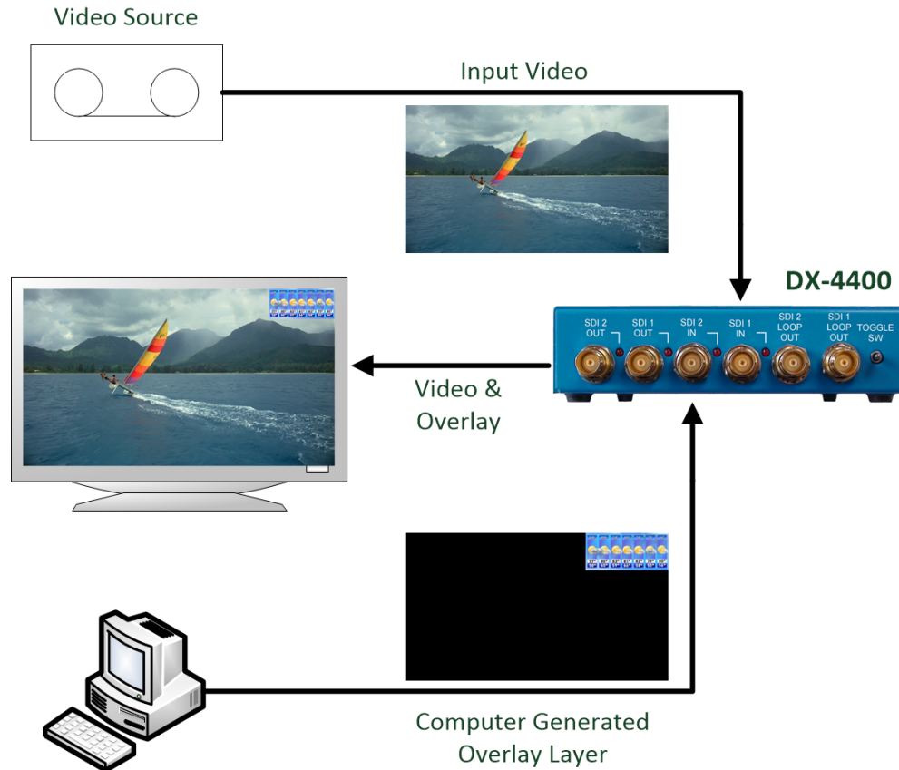
Figure 16: Example of Computer-generated Graphics Overlay with Transparency
