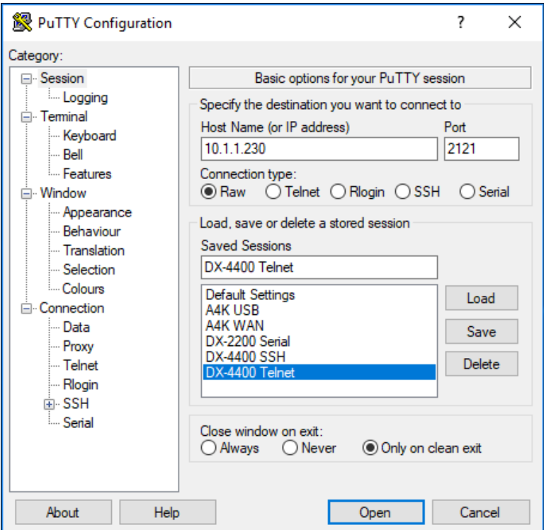
Figure 74: PuTTY TCP/IP Session Settings
