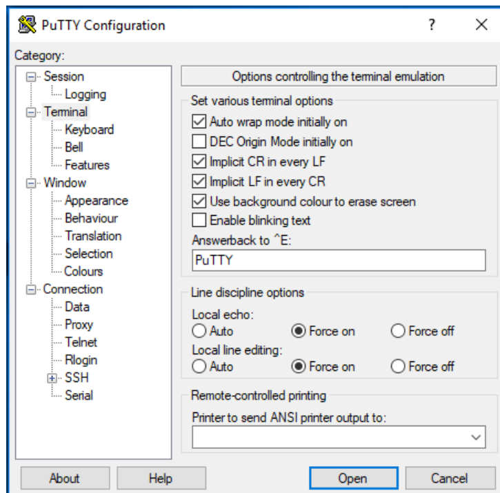
Figure 72: PuTTY Serial Port Terminal Settings
