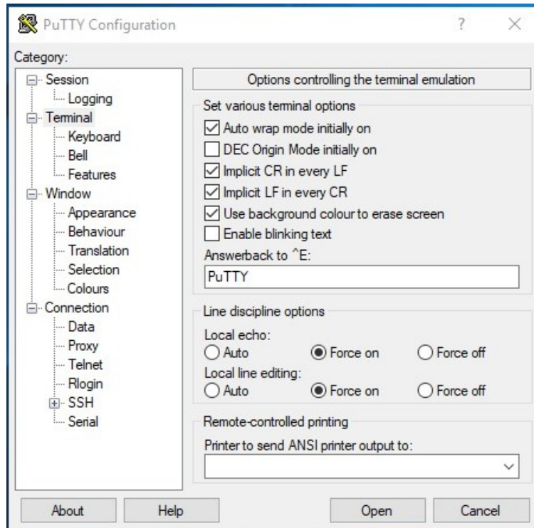
Figure 75: PuTTY Terminal Settings
