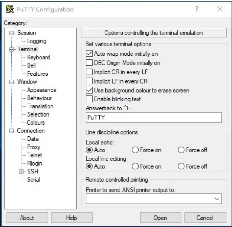
Figure 77: PuTTY SSH Terminal Settings
