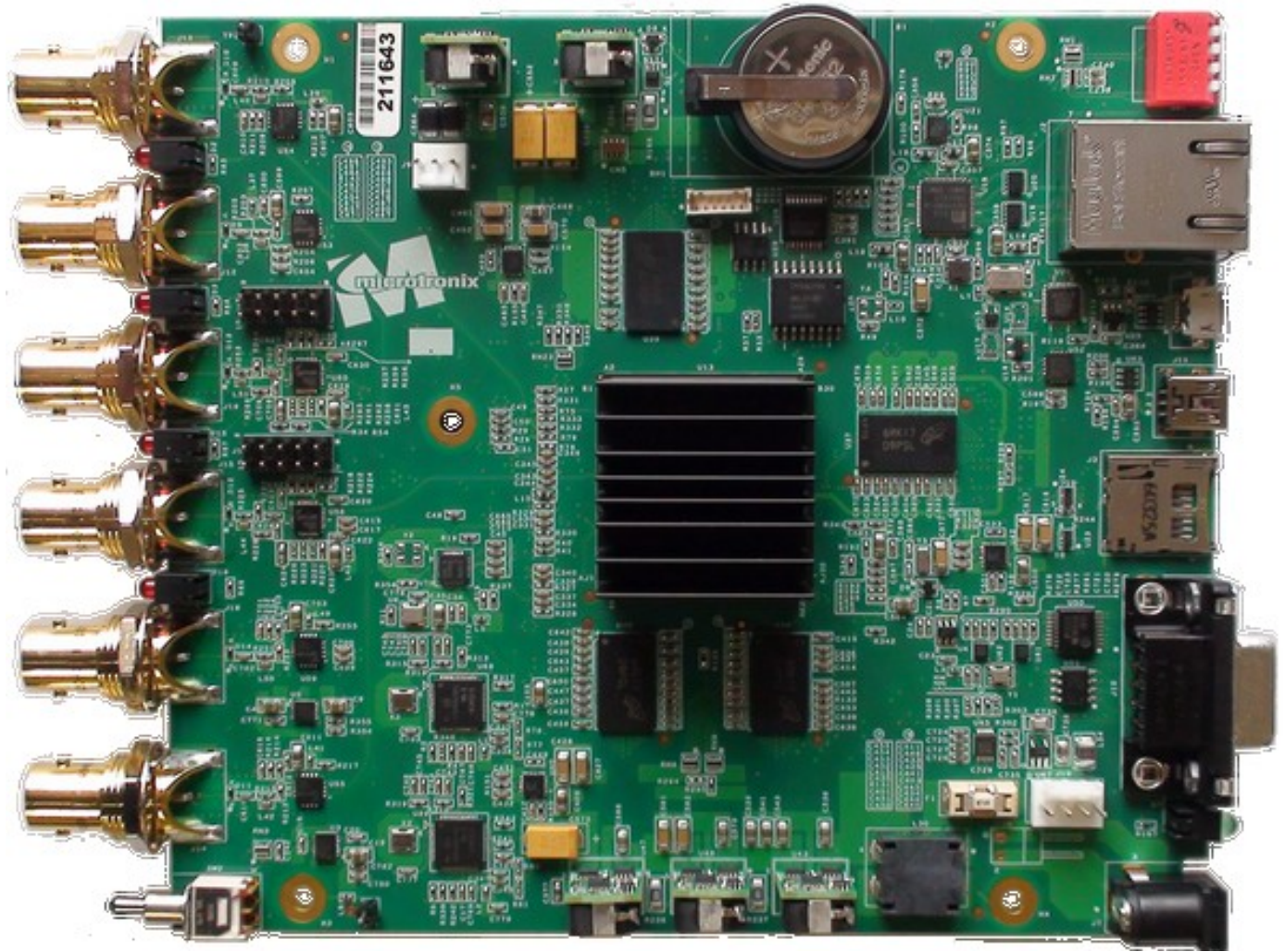
Figure 68: DX-4400 – SD/HD/2K/4K-SDI Text & Graphics Overlay Inserter OEM Board
