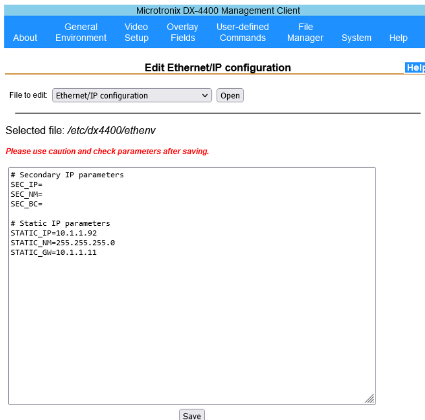
Figure 9: ethenv Configured for Static IP
