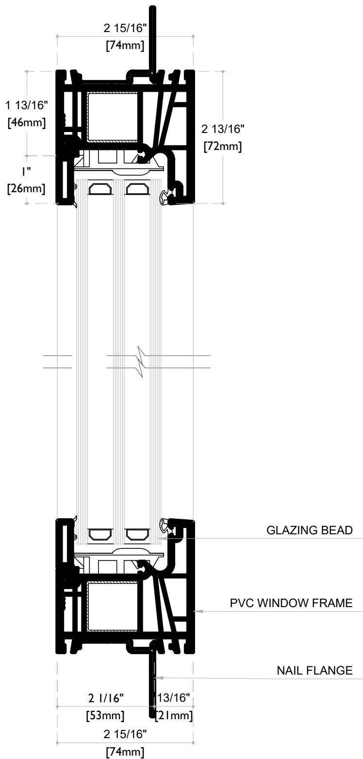
04 PROFILE DETAIL A-02 SCALE: N/S
