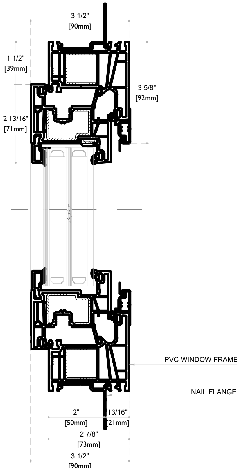
04 PROFILE DETAIL A-03 SCALE: N/S
