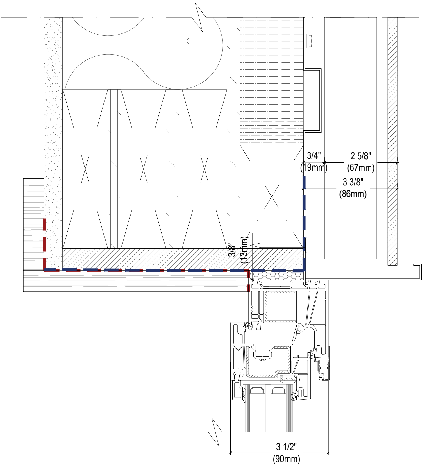
01 WINDOW HEAD DETAIL A-03 SCALE: 6"=1'-0"
