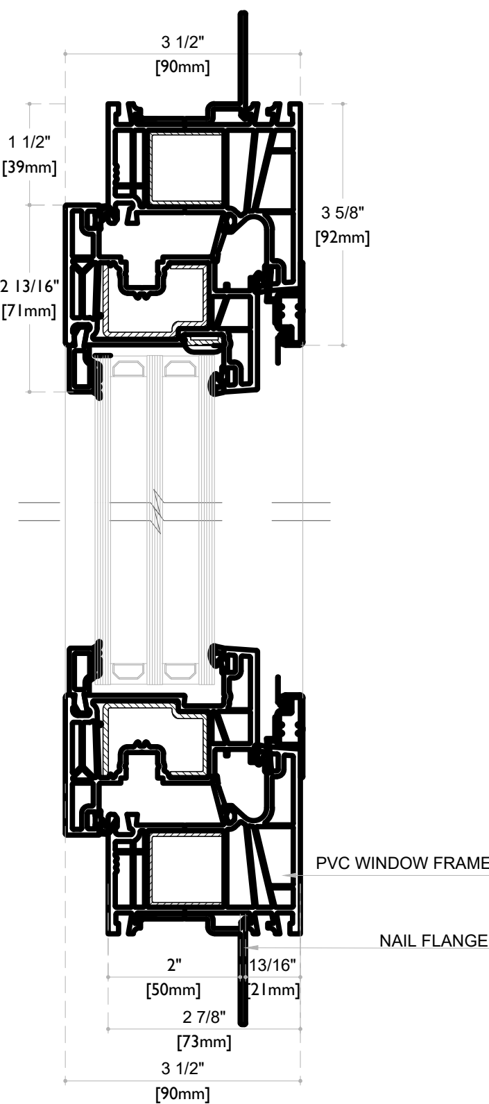
04 PROFILE DETAIL A-04 SCALE: N/S
