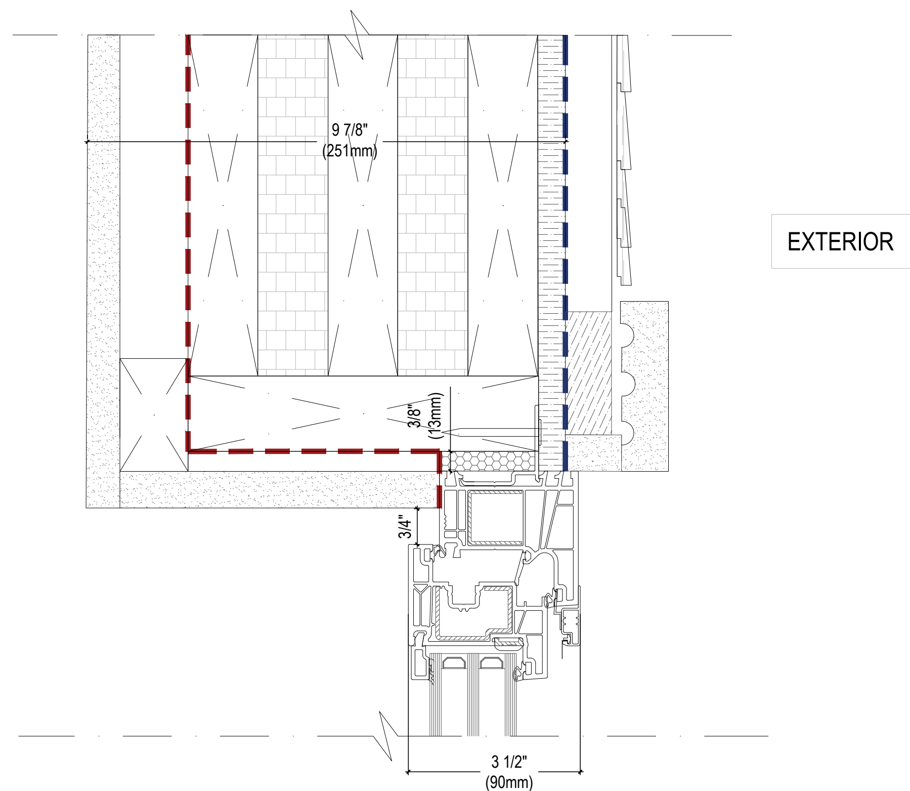
01 WINDOW HEAD DETAIL A-04 SCALE: 6"=1'-0"
