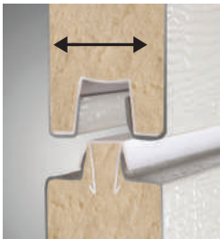
Cross Section
