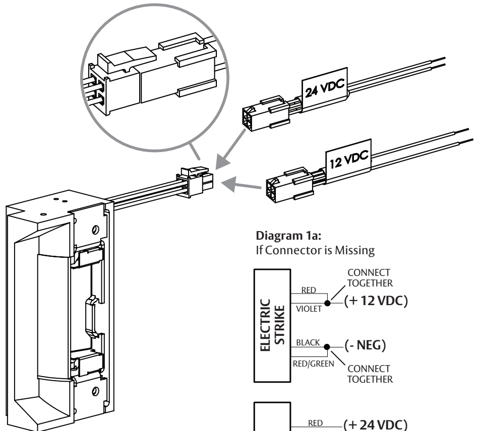
Diagram 1: 12 VDC to 24 VDC Conversion
