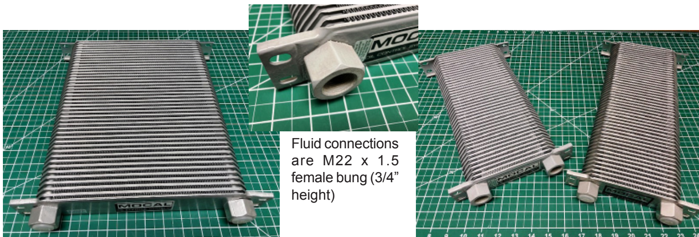
44 Row 235mm (series 6) Oil Coolers
