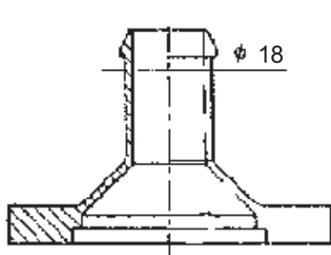
18mm (.70") push-on
