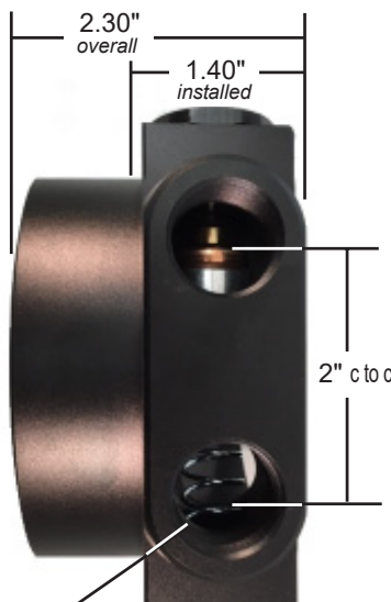
M22 x 1.5 thread ports (2)
