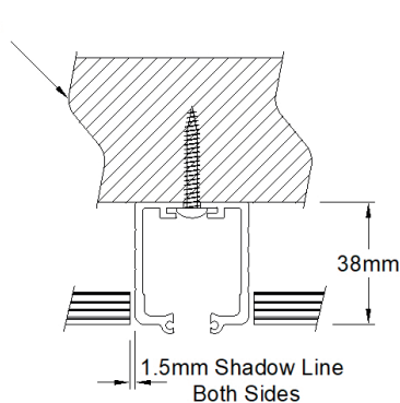
Recessed Track
