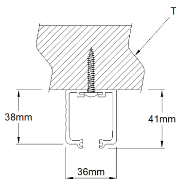
Exposed Track
