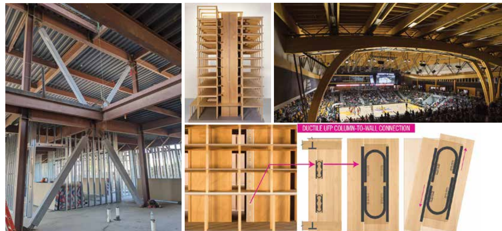
Cross Laminated Timber (CLT) is gaining momentum in various design and structural applications throughout the West. (top-right) Exposed beams provide a bold engineering statement at the Idaho Central Credit Union Arena in Moscow, Idaho (photo courtesy KPFF). Renderings of a rocking CLT wall system illustrate how fuses help to dissipate energy in a seismic event (renderings by Lever Architects). Traditional steel structural systems are shown (left) in this under construction image (photo courtesy Dunn Associates, Inc.)
