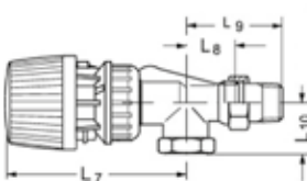
Horizontal Angle RA-N 10, 15, 20 & RA-FN 10 or 20
