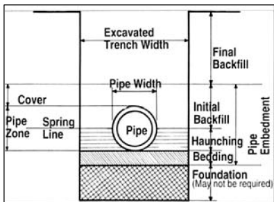
Figure 1 Trench Terminology
