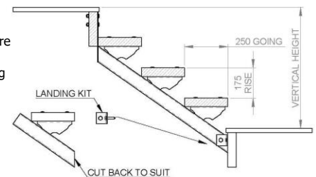
LANDING TO LANDING STAIR STRINGER
