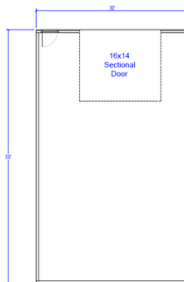
Building 2 - 30x50 (1,500 sq ft)
