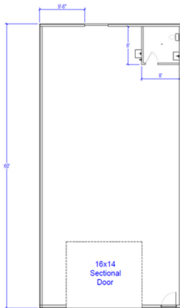
Building 1 - 30x60 (1,800 sq ft)
