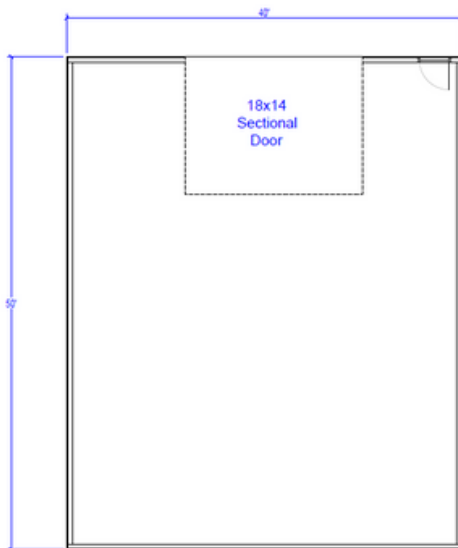
Building 2 - 40x50 (2,000 sq ft)
