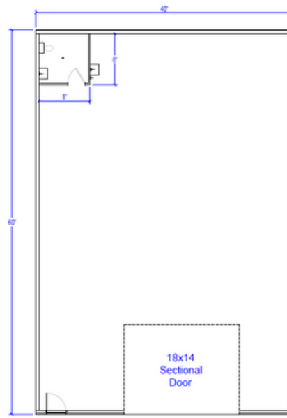
Building 1 - 40x60 (2,400 sq ft)
