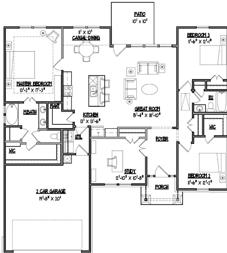
Floor Plan
