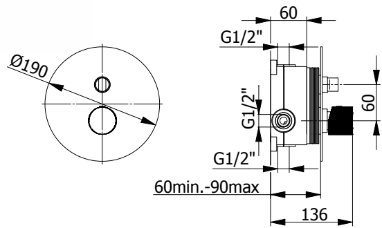
PC04055 Cartuccia Ø35mm Ø35mm cartridge
