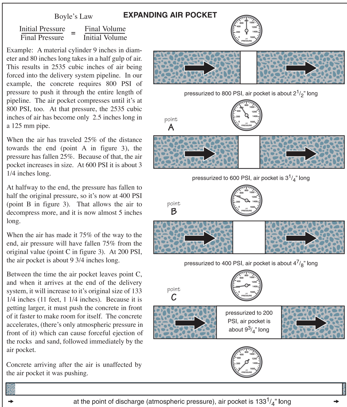
Figure 5 Air expands as pressure drops
