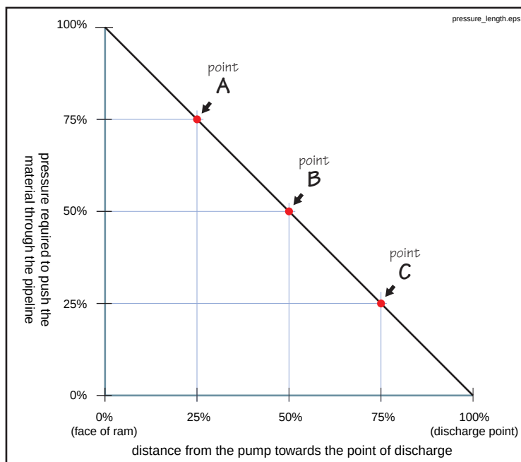
Figure 3 Pressure as a function of distance
