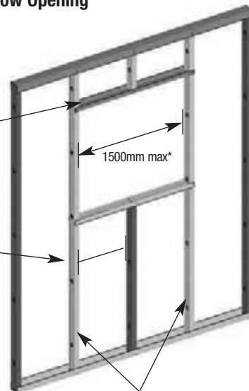
Fig. 2 Window Opening
