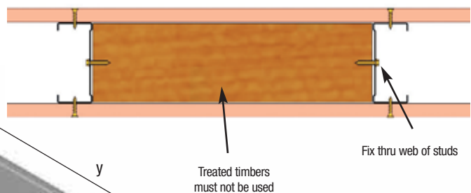
Fig. 3 Timber Nogging
