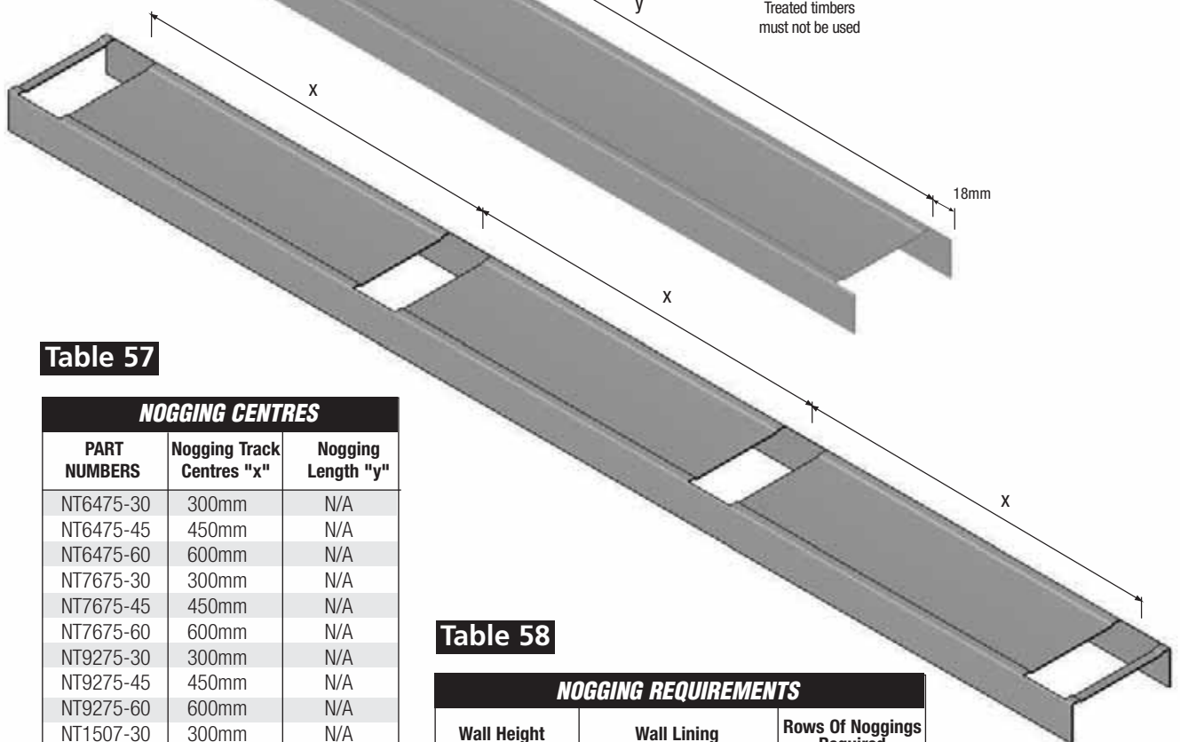
Fig. 2 Nogging Track
