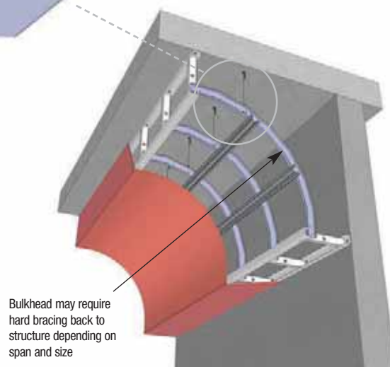
Fig. 5 Suspension of Prefabricated Bulkheads
