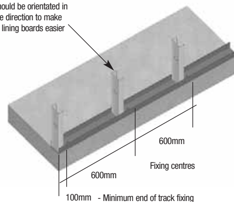
Fig. 2 Fixing Centres
