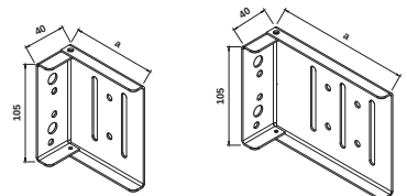
M190 Bypass Framing Connector
