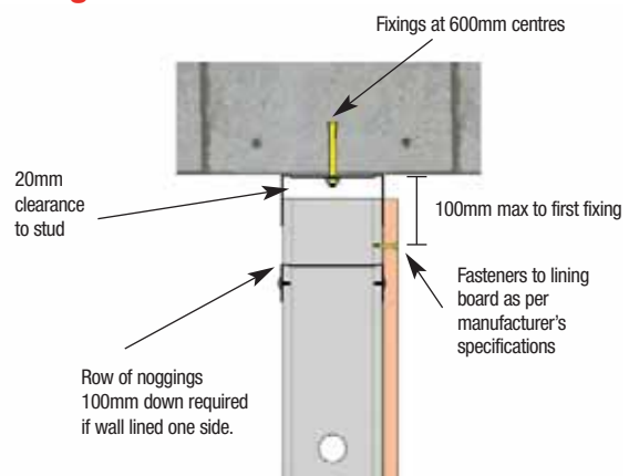
Fig. 4 Deflection Head
