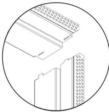
Locate fixing tabs to header.
