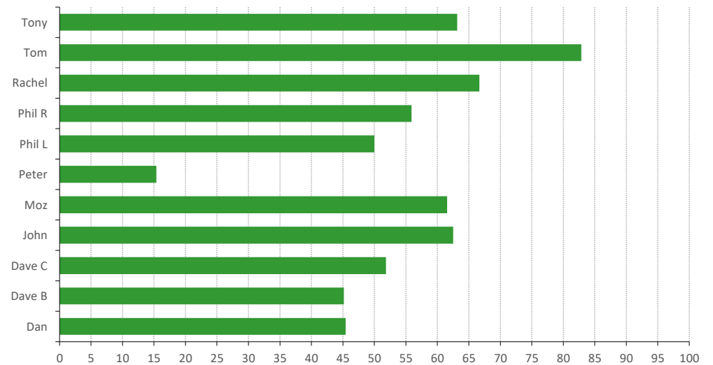
Percentage WON
