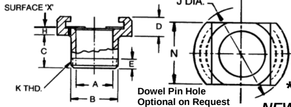
TYPE HNL
