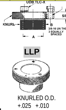
LOCK RING
