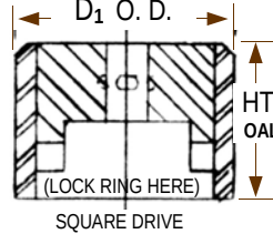
SQUARE DRIVE
