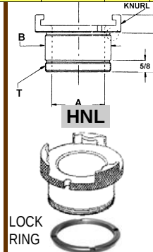
KNURLED O.D. +.025 +.010
