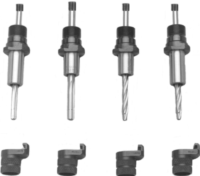
Coolant Oil Hole Threaded Shank Reamers
