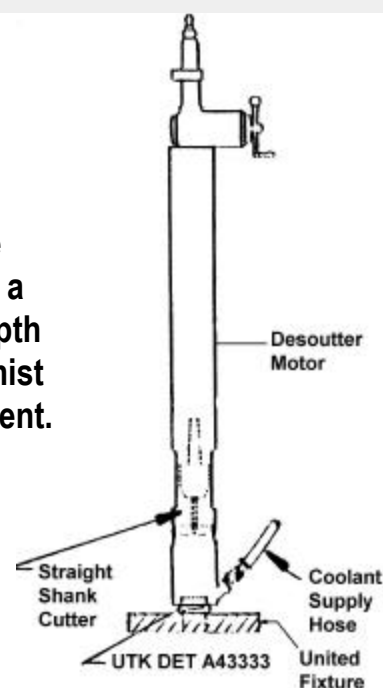
Typical Set Up with Drill Motor and UNITED s Coolant Nosepiece.
