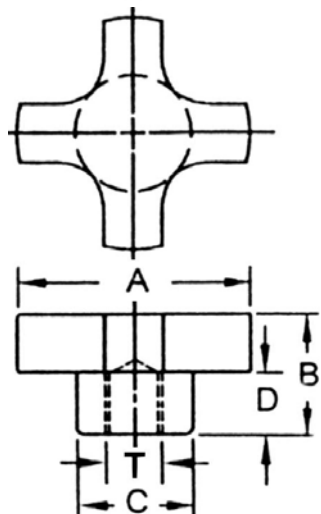
MOLD-IN BRASS INSERT
