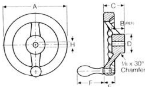
DIAMETERS FROM 4 TO 10 INCHES
