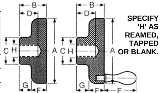
WITHOUT HANDLE STYLE
