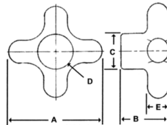
UnEcon Cast Iron Hand Knobs — INCH & METRIC SIZES
