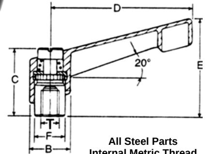
TAPPED TYPE A
