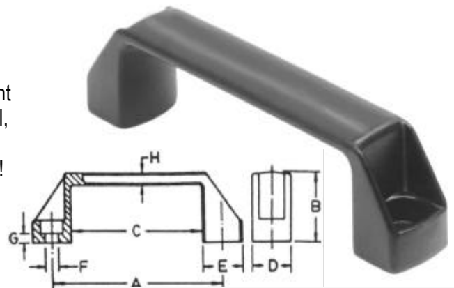
RECTANGULAR CABINET
