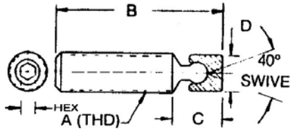
SWIVEL SCREW CLAMP WITH SMALL FOOT
