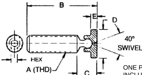
SWIVEL SCREW CLAMP WITH LARGE FOOT
