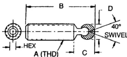
SWIVEL SCREW CLAMP WITH ROUND FOOT
