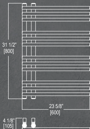
Horizontal Tube
