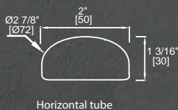
Horizontal tube
