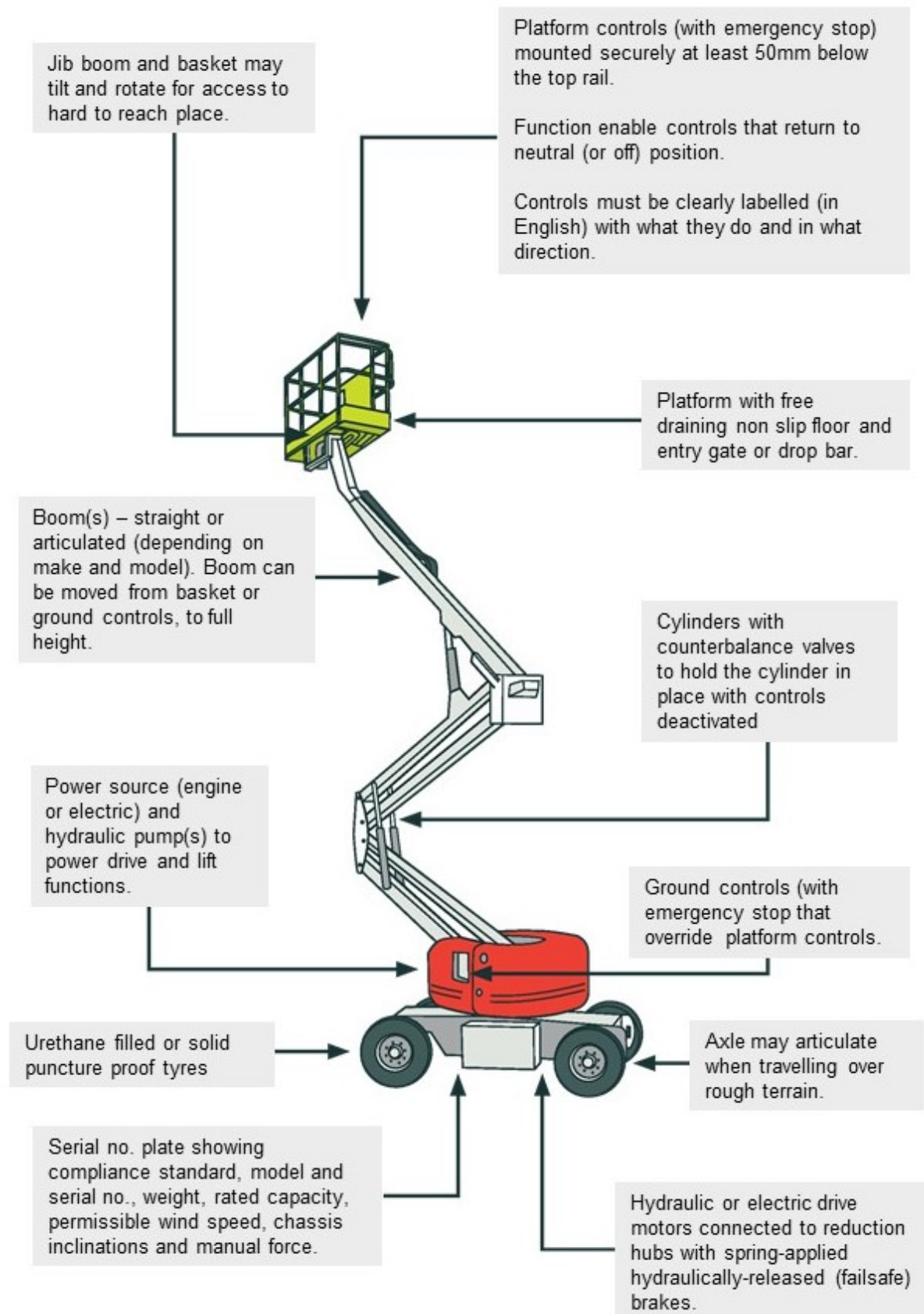
Figure 7: Typical Features of a Self-Propelled Boom Lift.
