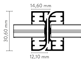
profilo verticale di chiusura tra pannelli closing vertical profile between panels
