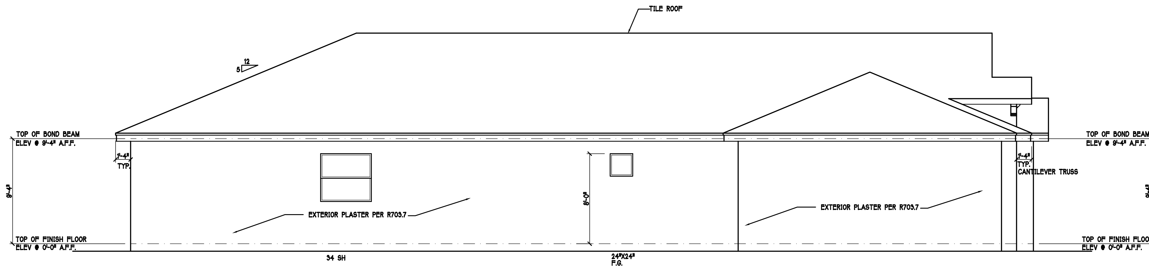
LEFT SIDE ELEVATION: "L" SCALE: 3/16" = 1'-0"
