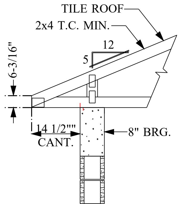
TYP. ROOF TRUSS END DETAIL N.T.S.
