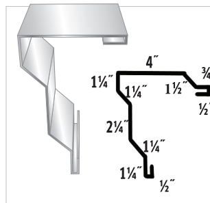
#32 Sculptured Rake
