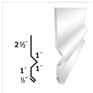
#43 Headwall Flashing
