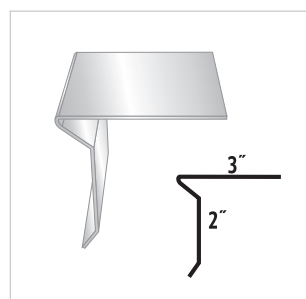
#45 Eave Trim
