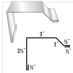
#24 Residential Rake
