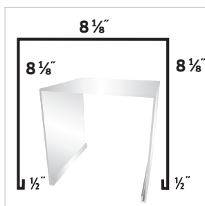
#86 8 x 8 Post Cover
