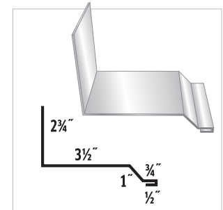
#11 Universal Sidewall
