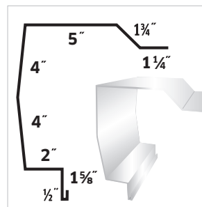
#88 Gable Trim
