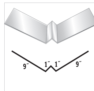
#25 Formed Valley
