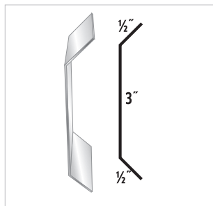
#41 Stucco Stop
