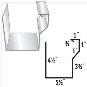
#56 Gutter
