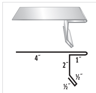
#22 "F" Trim
