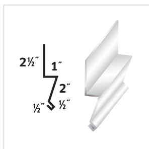
#90 Stucco Stop
