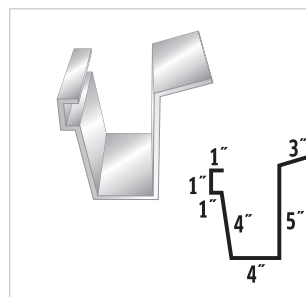
#50 Eave Gutter - Small
