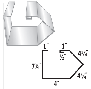
#55 Commercial Gutter
