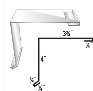
#49 Gable Rake Trim
