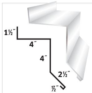
#74 Overhead Door Trim
