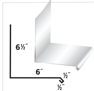
#28 "L" Flashing
