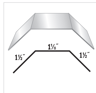
#58 PBR Gutter Hanger
