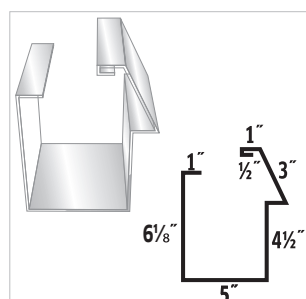
#54 Commercial Gutter
