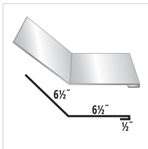
#67 Transition Flashing
