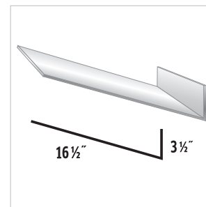
#81 Chimney Flashing
