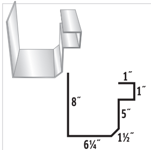
#52 Commercial Gutter
