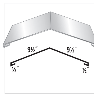
#40 XL Standard Ridge
