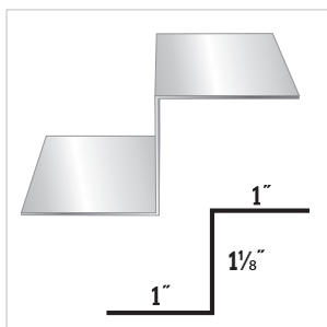
#48 Z Flashing
