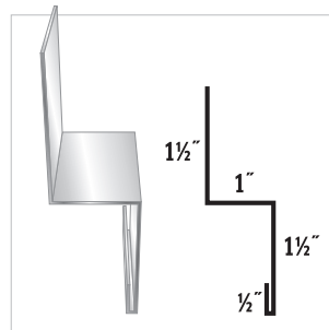
#10 Double Angle
