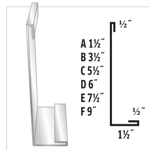
#14 Angle Trim
