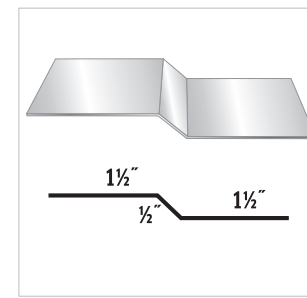
#30 Offset Cleat
