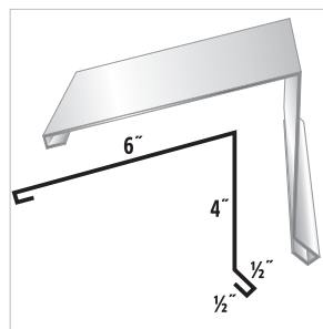
#80 Peak Cap
