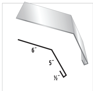
#27 Notched Gambrel
