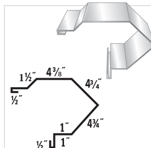
#33 Commercial Rake
