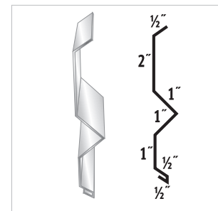
#34 Headwall Counter Flashing
