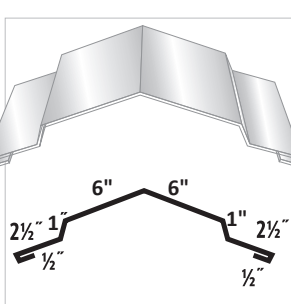
#39 XL Universal Ridge Cap
