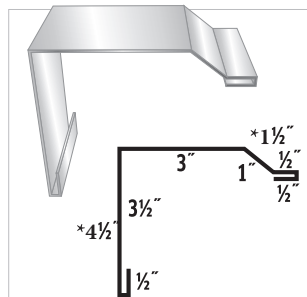
#31 Extended Rake (AG) #79 Extended Rake (*PBR)
