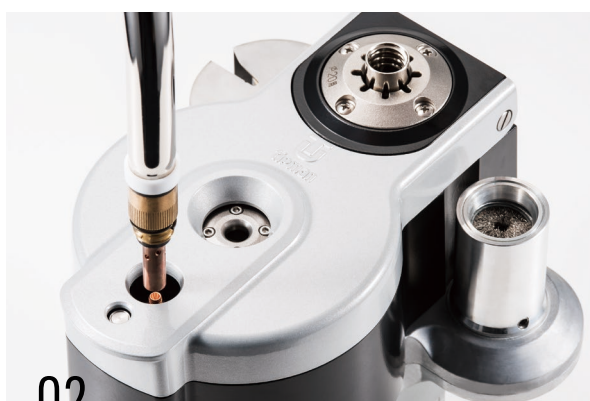
02 Functions of contact tip and nozzle removal. In regard to contact tip and nozzle attachment, the rotation automatically stops when the specified torque has been reached. Old contact tips are also collectable.
