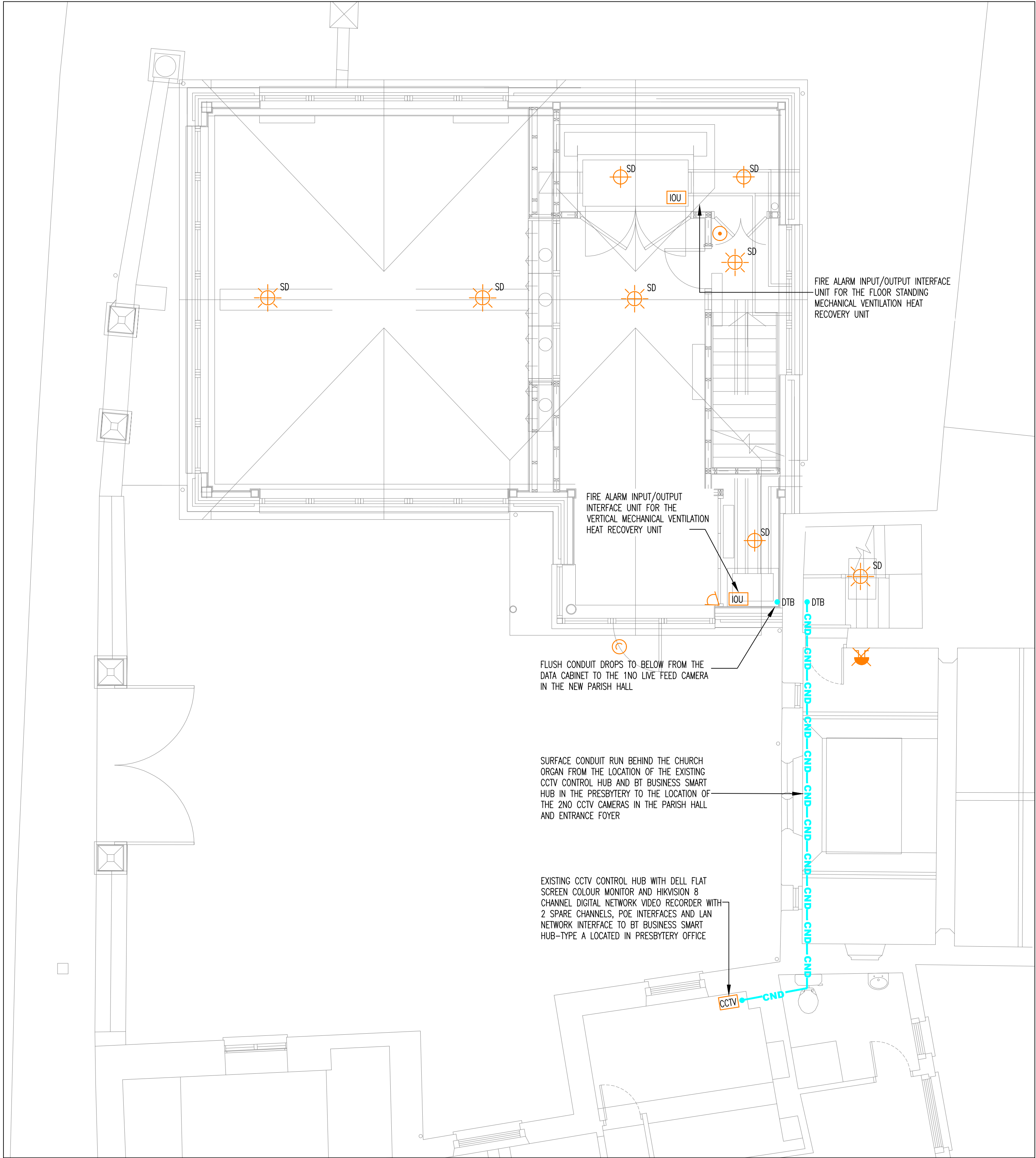
FIRST FLOOR
