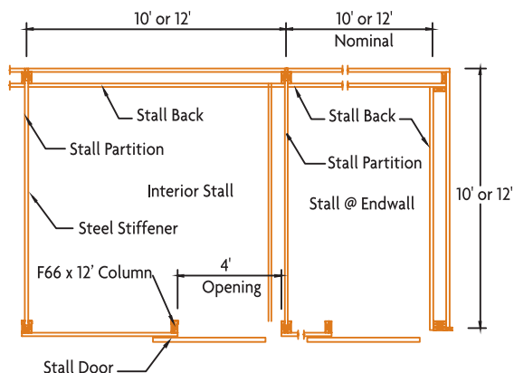
Stall Plan View Cribbing angles are standard at column edges.
