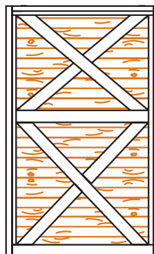
Solid 2x8 Tongue & Groove Plank w/ Crossbucks
