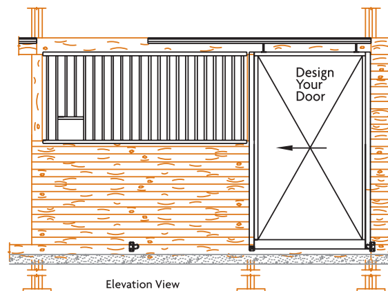
Solid 2x8 Tongue & Groove Plank With Upper Grill Section Cribbing angles are standard at column edges.
