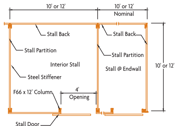
Stall Plan View Cribbing angles are standard at column edges.
