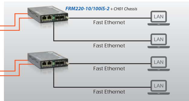
Customer Premise Equipment (CPE)
