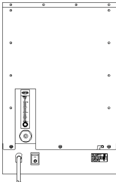
Shown: ClearWater Tech OXS100 Air Prep. Module (drawings not to scale)
