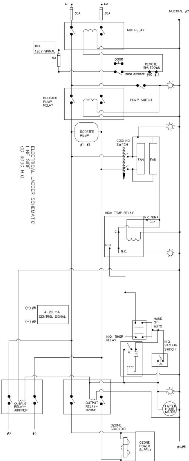
Shown: Electrical Schematic - CD4000HO Line Side
