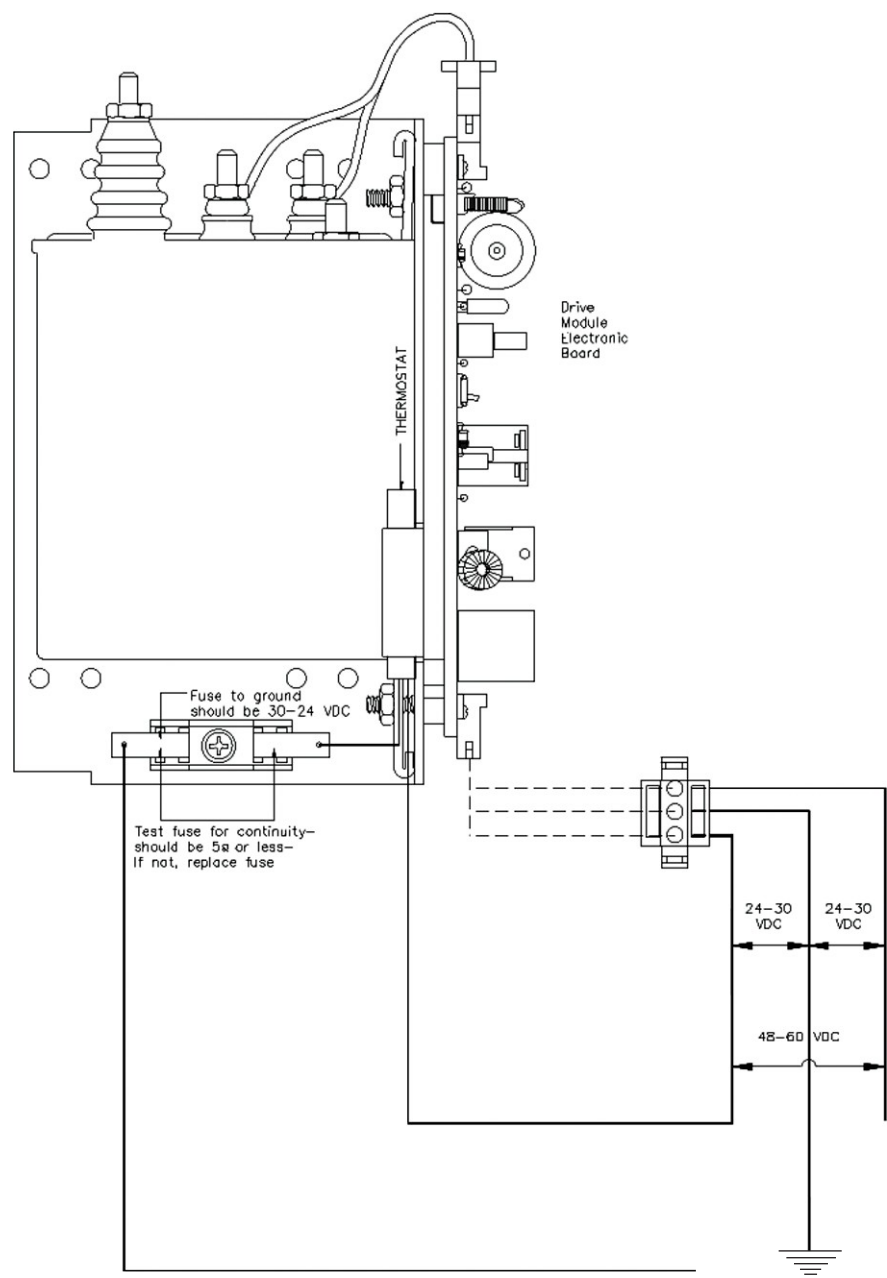
Shown: HO Drive Module
