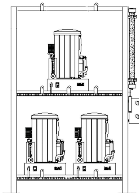
Shown: ClearWater Tech RMS45 Air Prep. System
