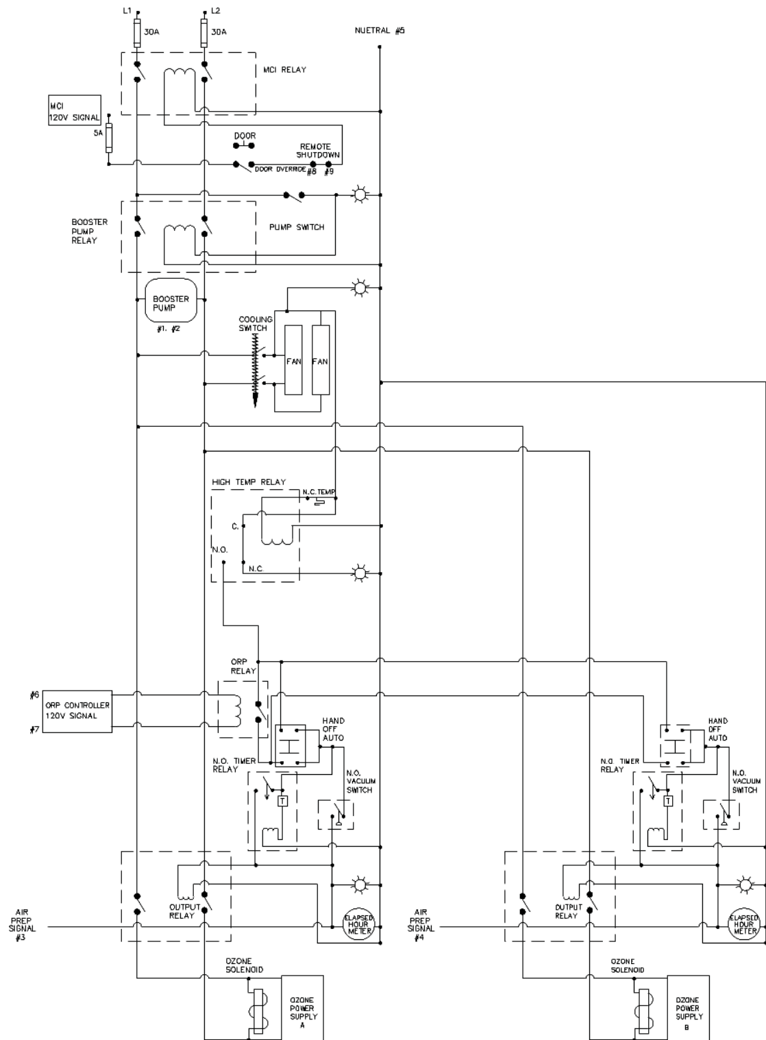
Shown: Electrical Schematic - CD-8000 and CD-12000 Line Side
