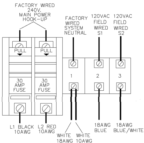
RMS-90 240 VAC, 50/60 Hz 1Ø, 17 amp system Figure 6-2 C For CD-12000 & CD12000HO
