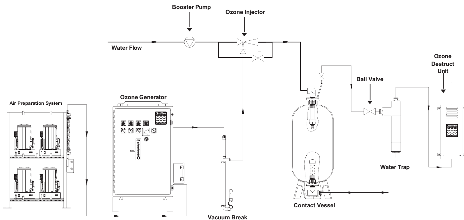
Shown: ClearWater Tech CD-8000HO Ozone System
