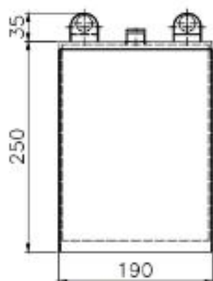
LEFT VIEW
