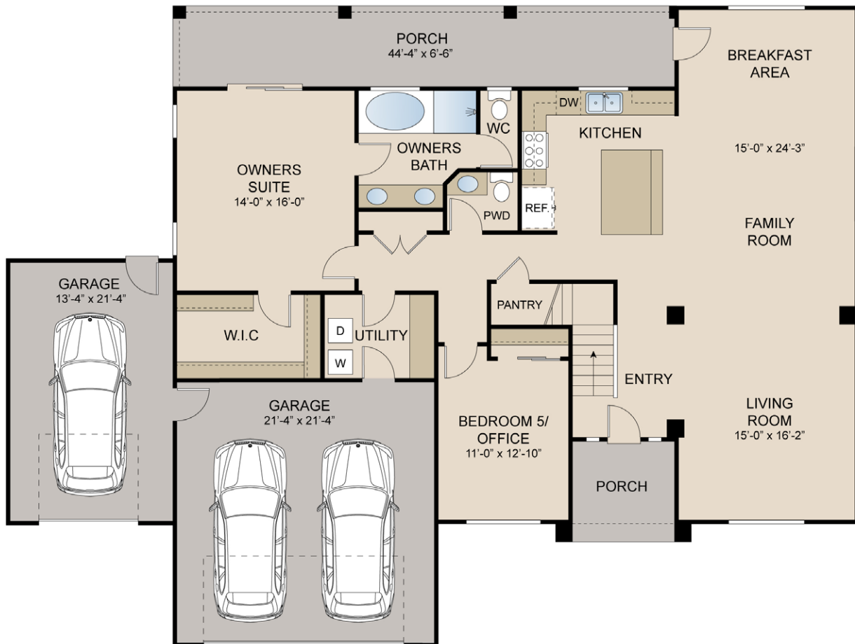
FIRST FLOOR
