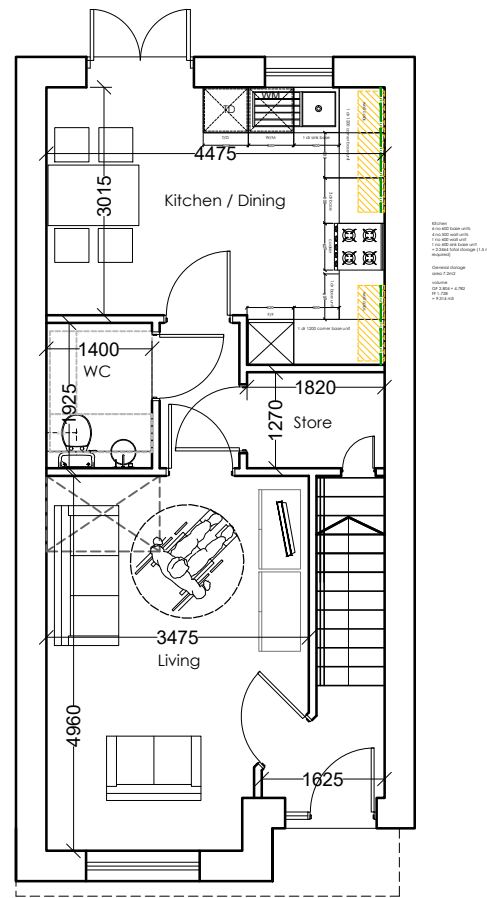
GROUND FLOOR PLAN (44m 2 / 474sq.ft.)
