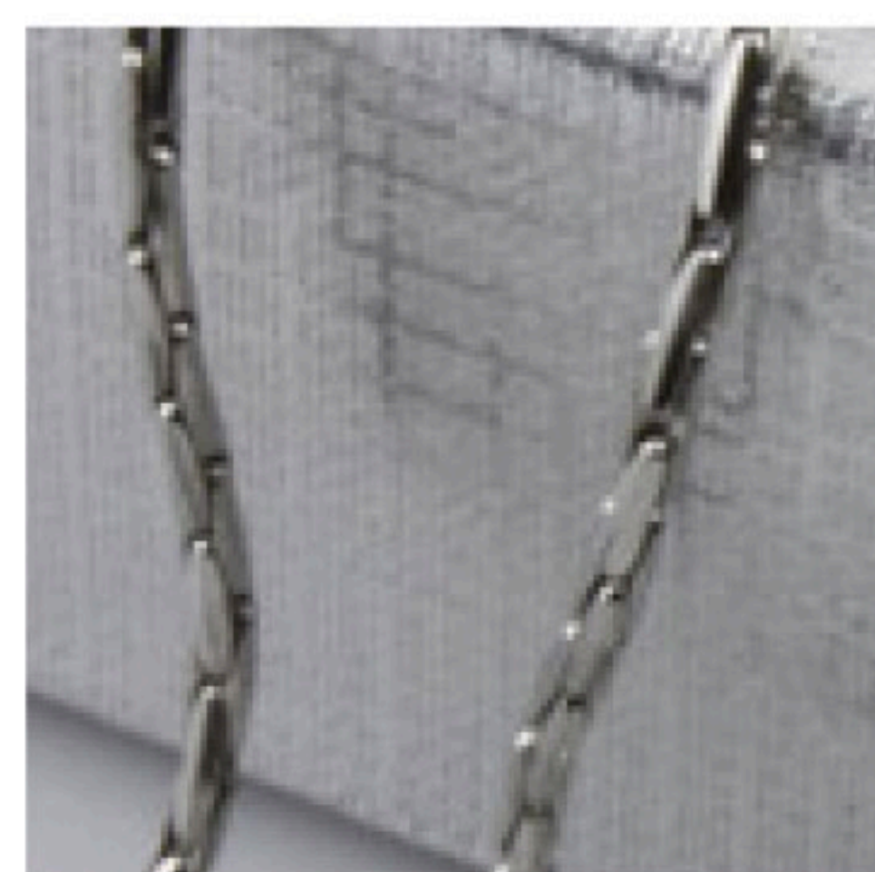
Block Chain
