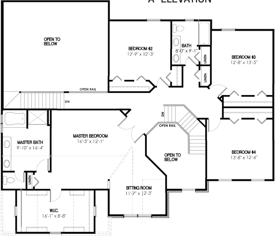
SECOND FLOOR “A” ELEVATION
