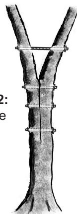
Figure 35.2.3: Alternating brace system
