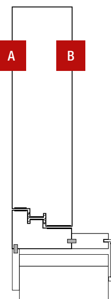
CERNIERE A SCOMPARSA INVISIBLE HINGES
