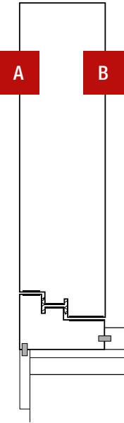
CERNIERE A SCOMPARSA INVISIBLE HINGES
