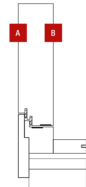
CERNIERE A SCOMPARSA INVISIBLE HINGES
