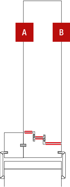
CERNIERE POMELLA BRASS HINGES
