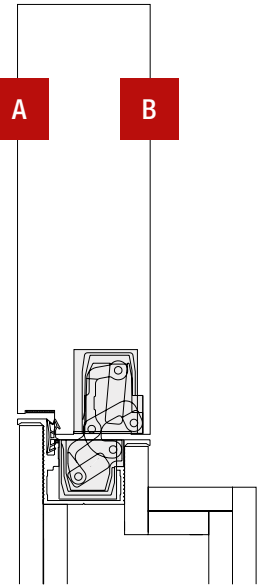
CERNIERE A SCOMPARSA INVISIBLE HINGES
