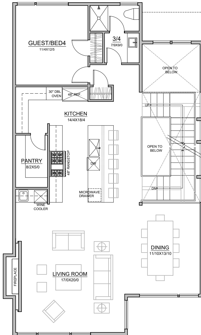
UPPER FLOOR PLAN 1,346 SQ.FT.
