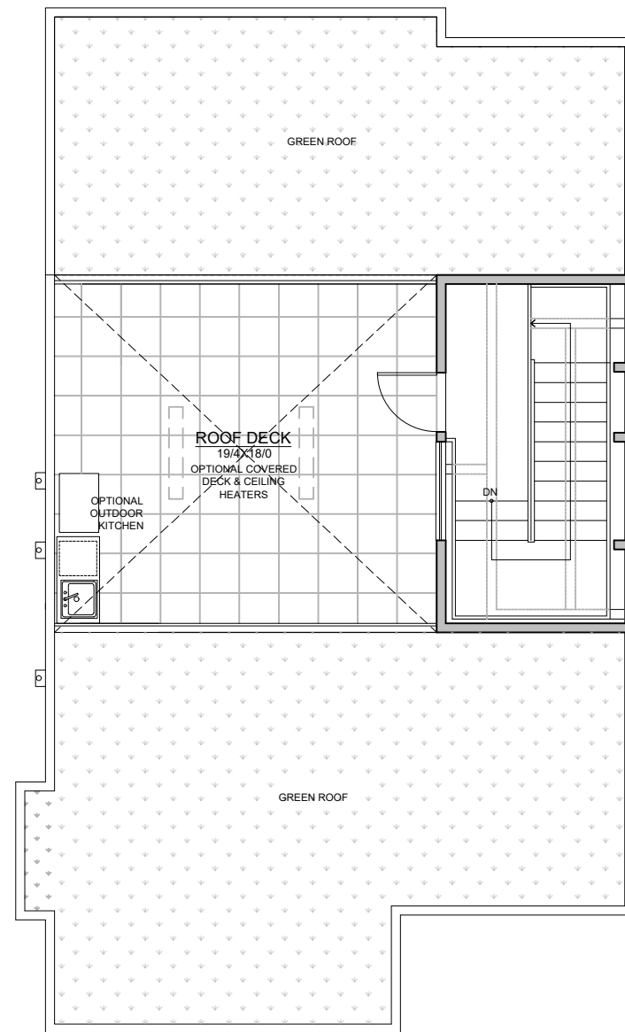
ROOF DECK 350 SQ.FT.
