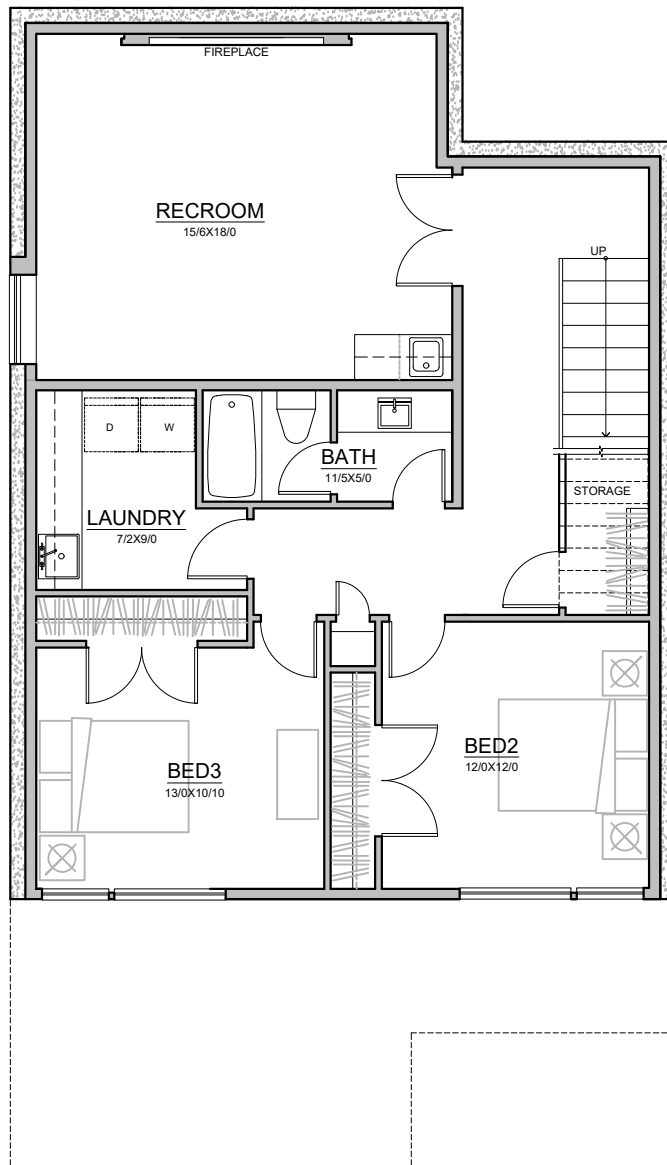
LOWER FLOOR PLAN 1,064 SQ.FT.
