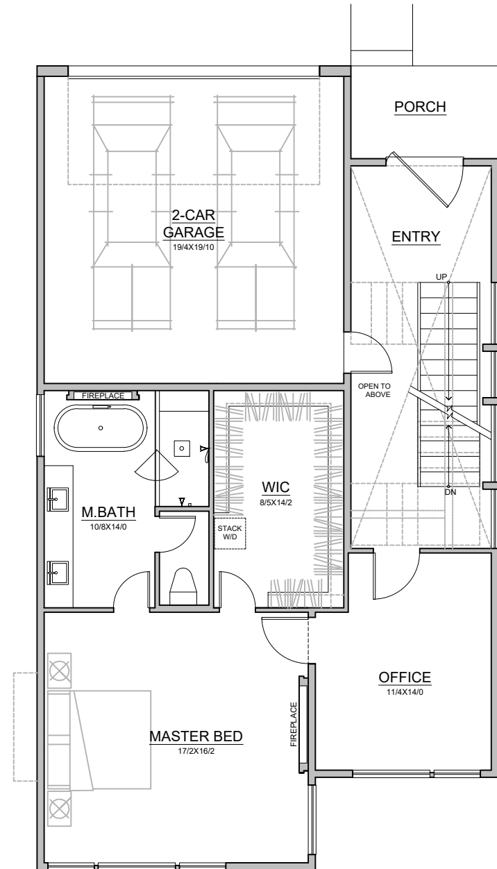
MAIN FLOOR PLAN 988 SQ.FT. TOTAL 3,400 SQ.FT.
