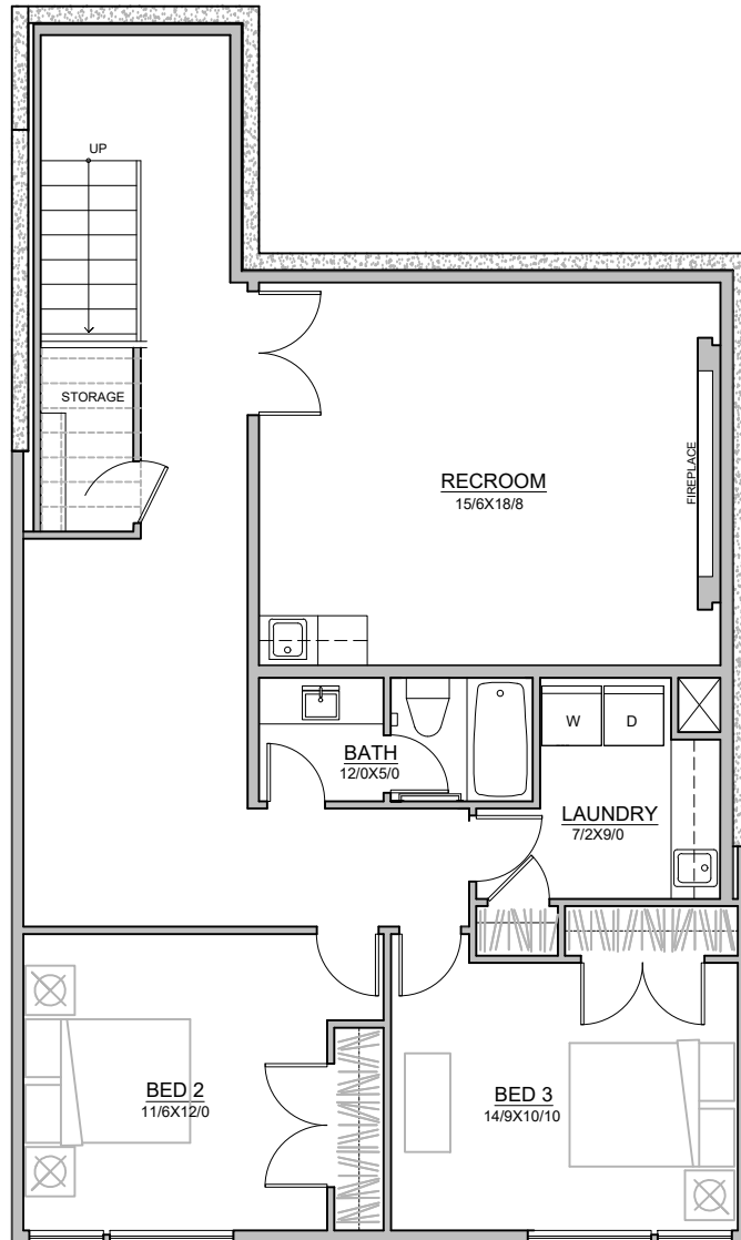
LOWER FLOOR PLAN 1,230 SQ.FT.
