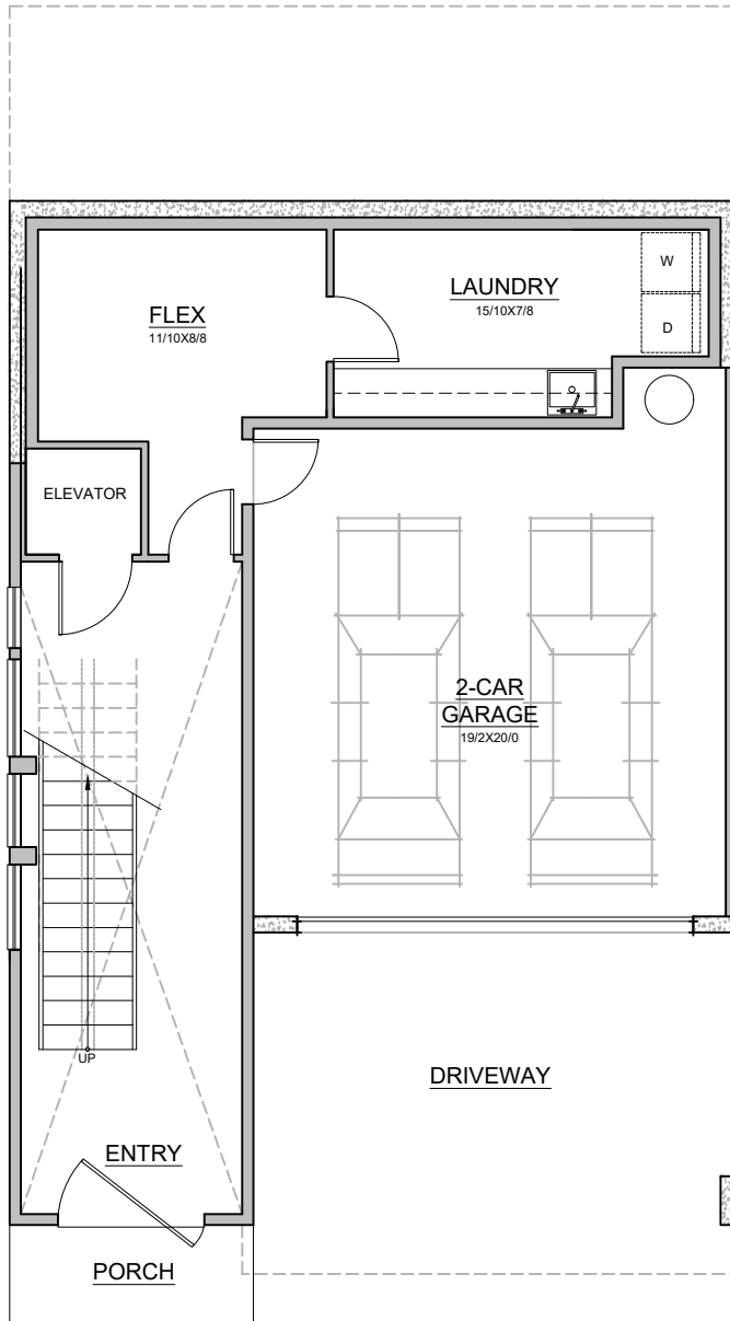
LOWER FLOOR PLAN 560 SQ.FT.
