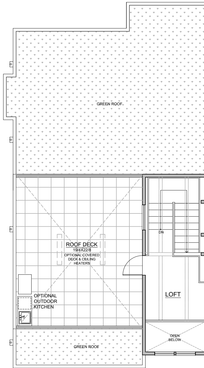
ROOF DECK 440 SQ.FT.
