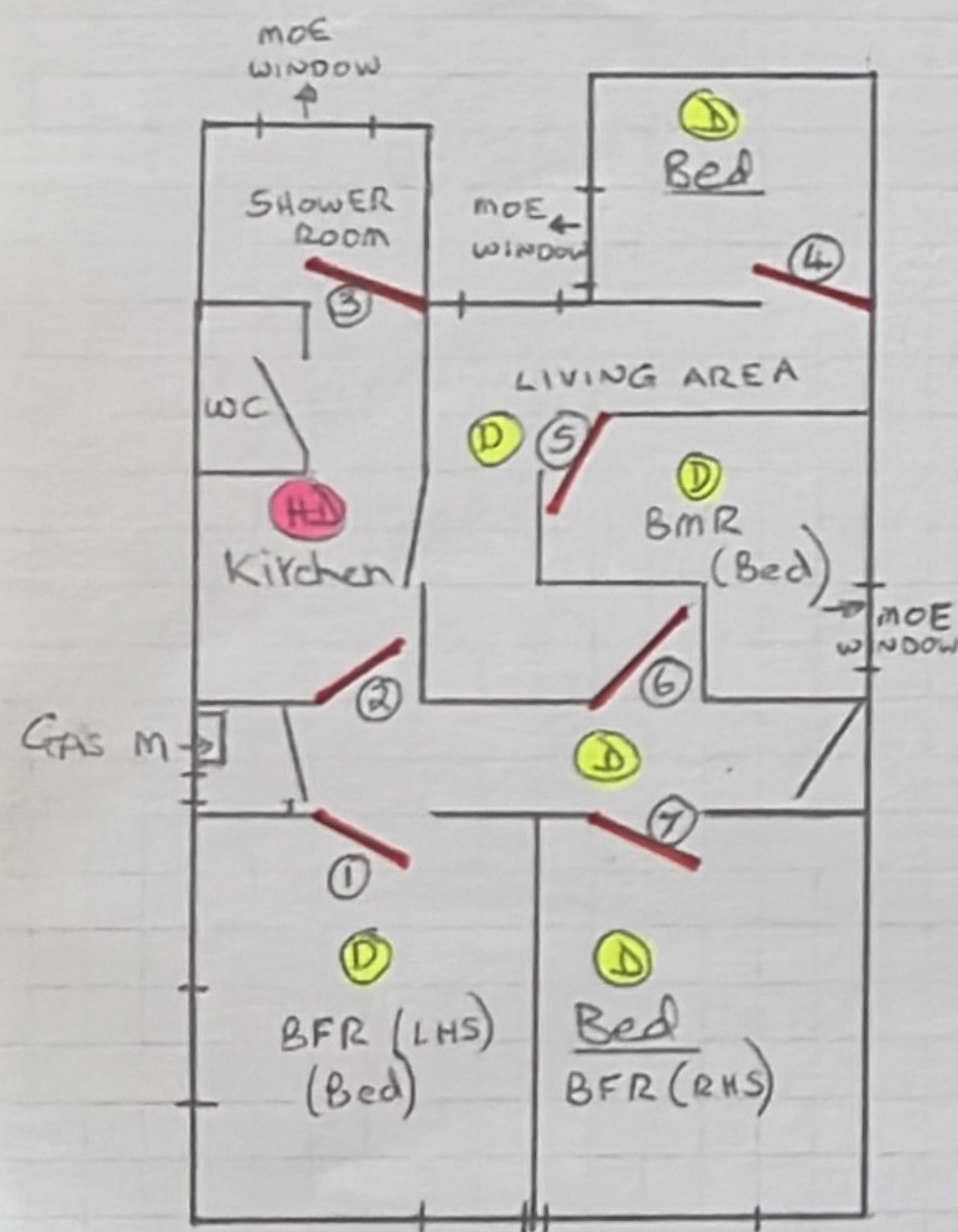
BASEMENT FLAT
