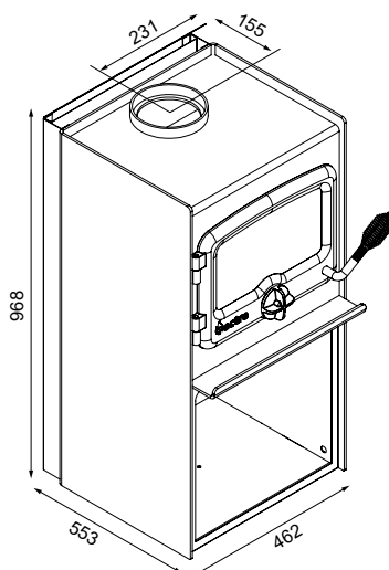
Wood Stacker
