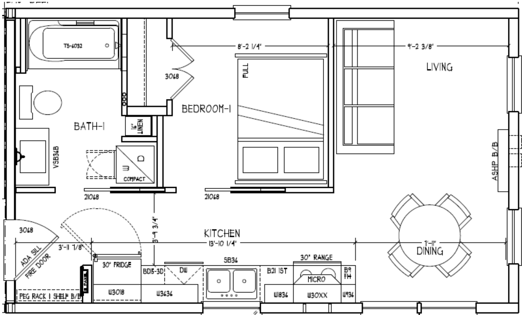
One Bedroom Layout (some units are mirrored) Unit 101, 201, 202, 203, 301, 302
