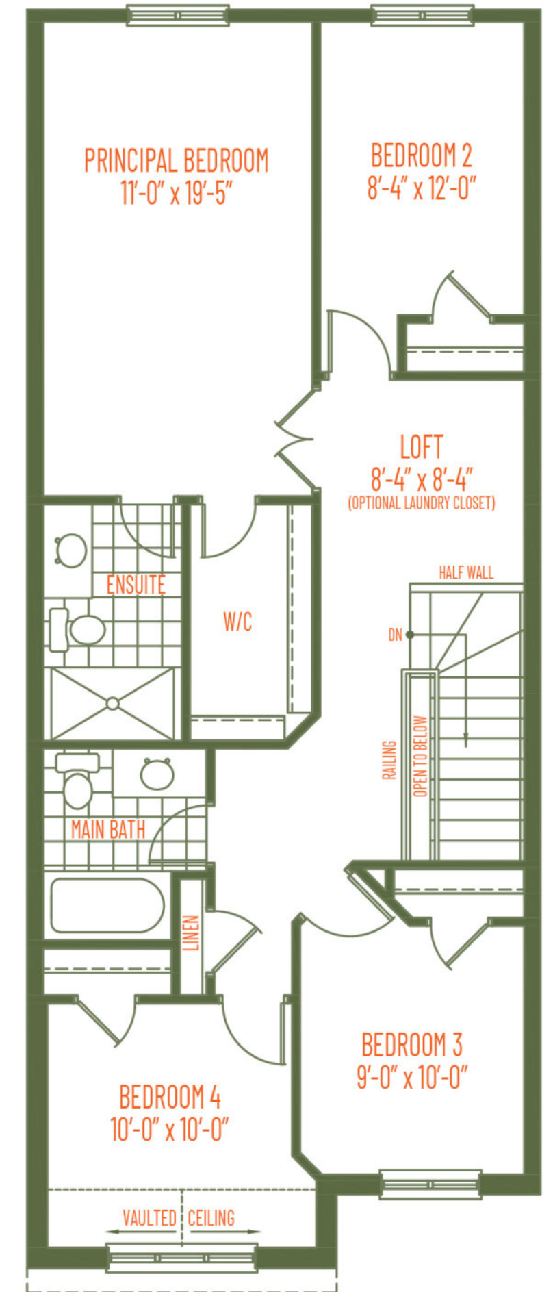
INTERIOR 4 BEDROOM SECOND FLOOR PLAN
